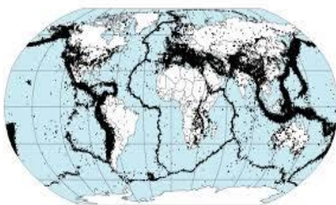
Preliminary Determination of Epicenters 358,214 Events, 1963 - 1998
